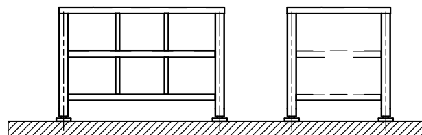
PANCHINA CASELLARIO PIGEONHOLE BENCH
